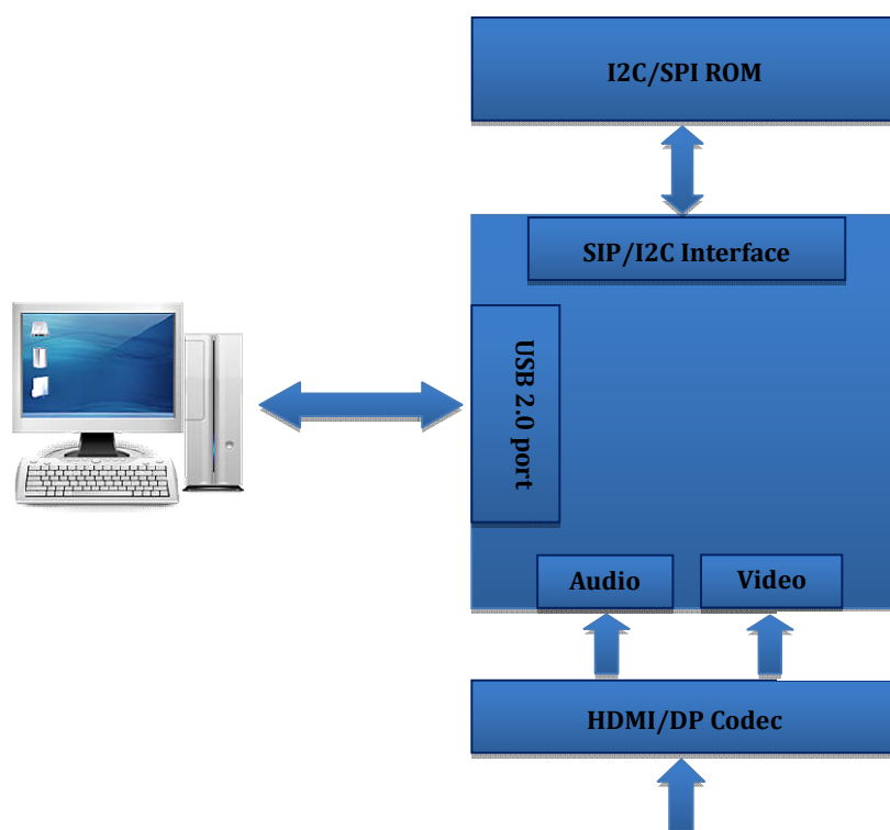
Figure 1-1. Application Diagram
