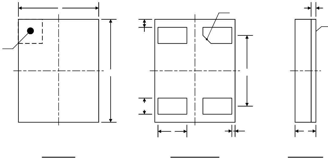
Figure 3.1. Package Outline Drawing
